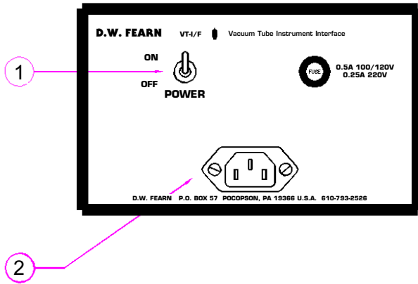
Figure 1. VT-I/F Rear Panel Connections and Controls
