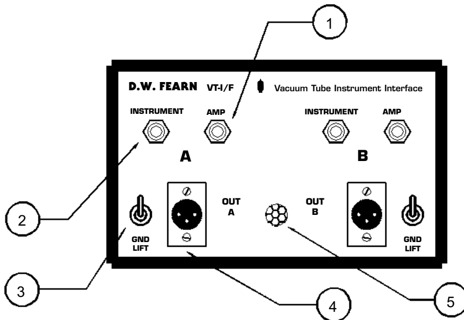
Figure 2. VT-I/F Front Panel Controls and Connections
